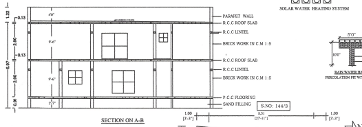
SECTION ON A-B
