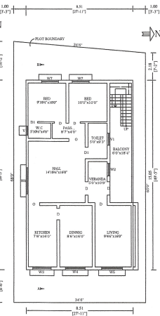
PRO. FIRST FLOOR PLAN
