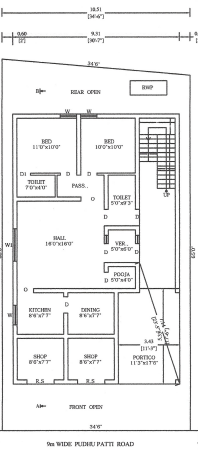
EXG. GROUND FLOOR PLAN
