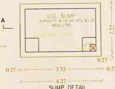
SUMP DETAIL SCALE 1" = 4'-0"
