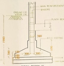
TYPICAL SECTION OF R.C.C. COLUMN FOUNDATION SCALE 1" = 2'-0"
