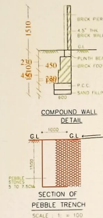
SECTION OF PEBBLE TRENCH SCALE 1" = 100
