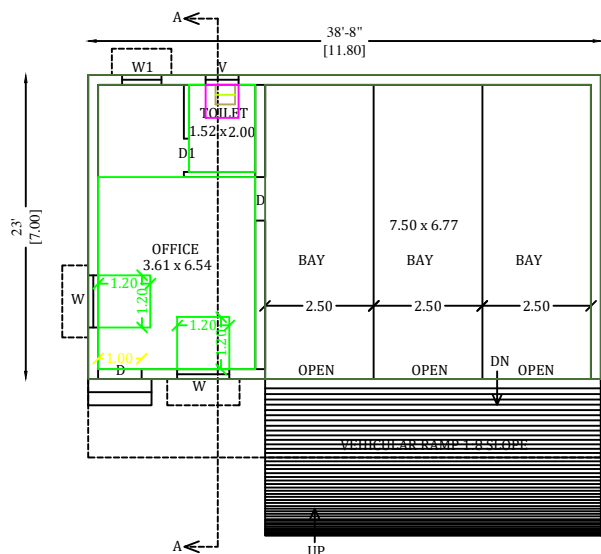
GROUND FLOOR PLAN (BLOCK-1)
