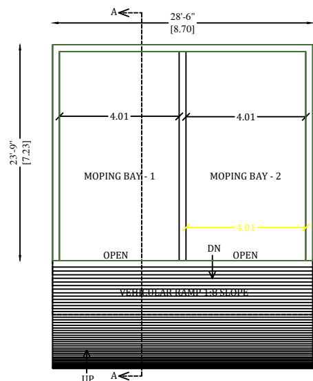
GROUND FLOOR PLAN (BLOCK-2)
