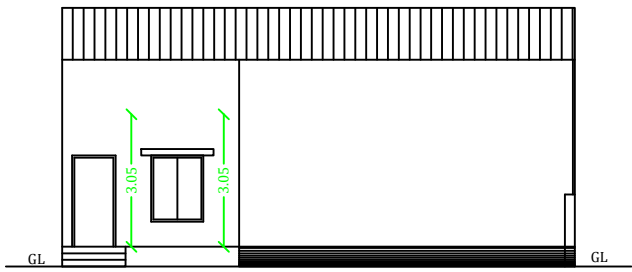
ELEVATION (BLOCK-1)
