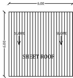
TERRACE FLOOR PLAN (BLOCK-3)
