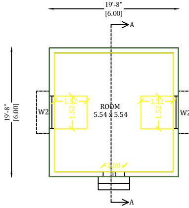
GROUND FLOOR PLAN (BLOCK-3)
