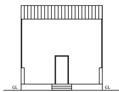
ELEVATION (BLOCK-3)
