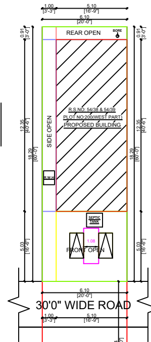
SITE PLAN
