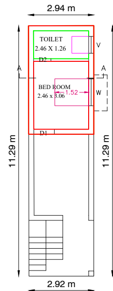
PRO.FIRST FLOOR PLAN
