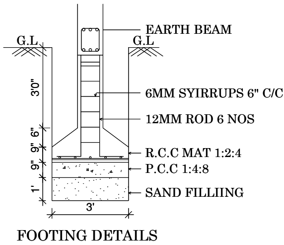
FOOTING DETAILS
