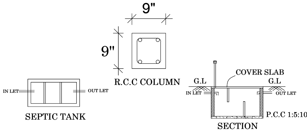
SECTION
