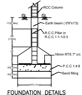
FOUNDATION DETAILS
