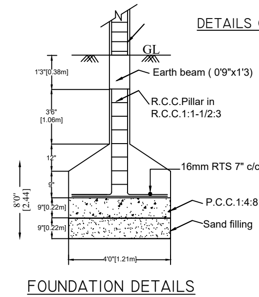
FOUNDATION DETAILS
