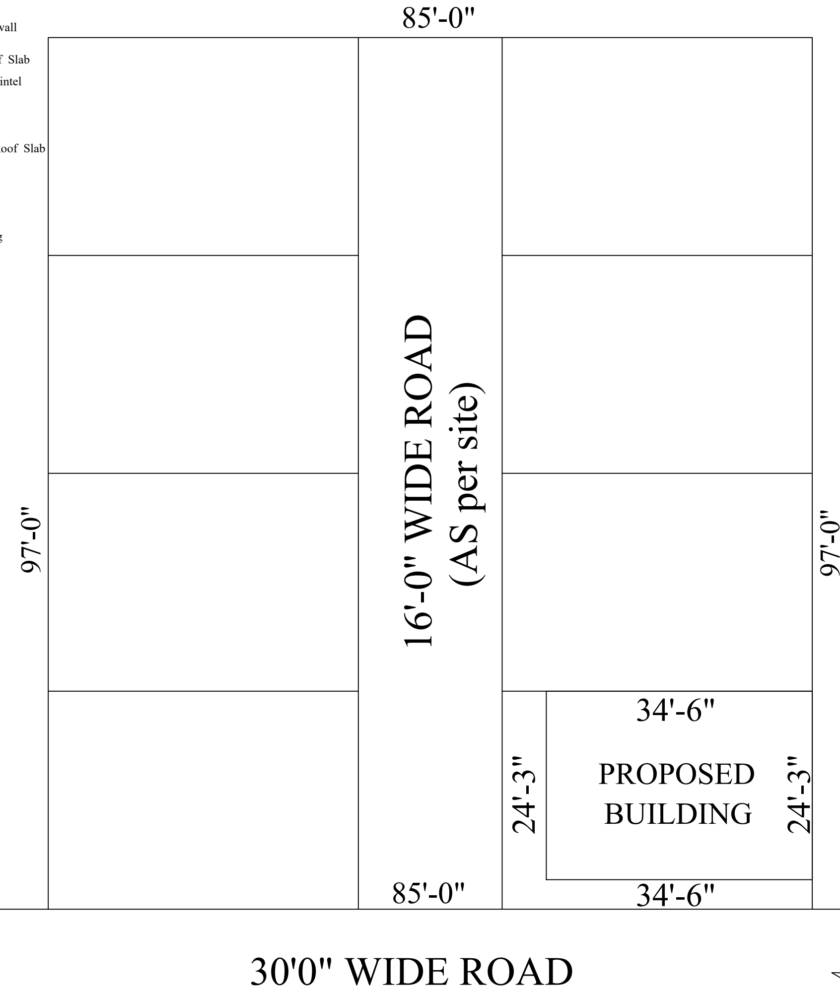
SITE PLAN
