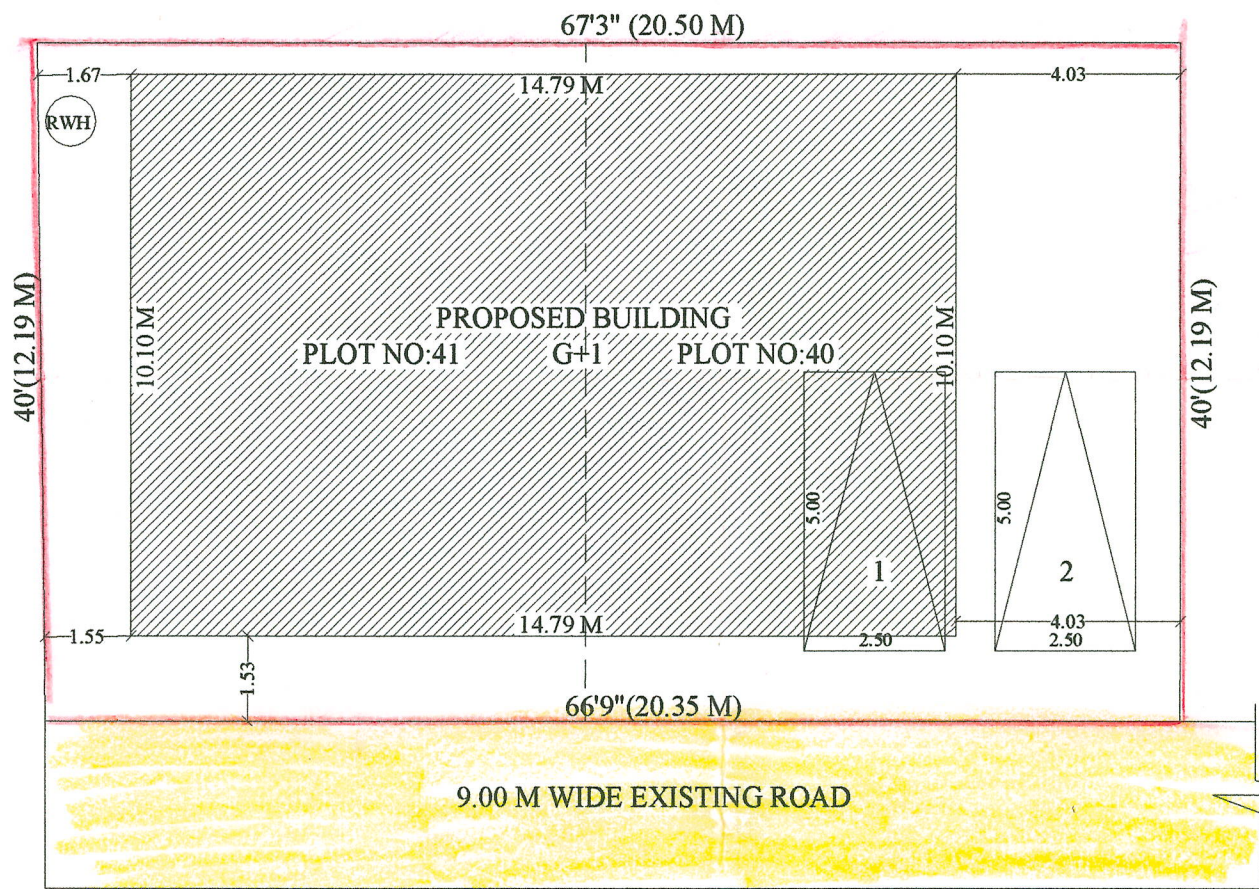
SITE PLAN
