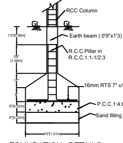
FOUNDATION DETAILS
