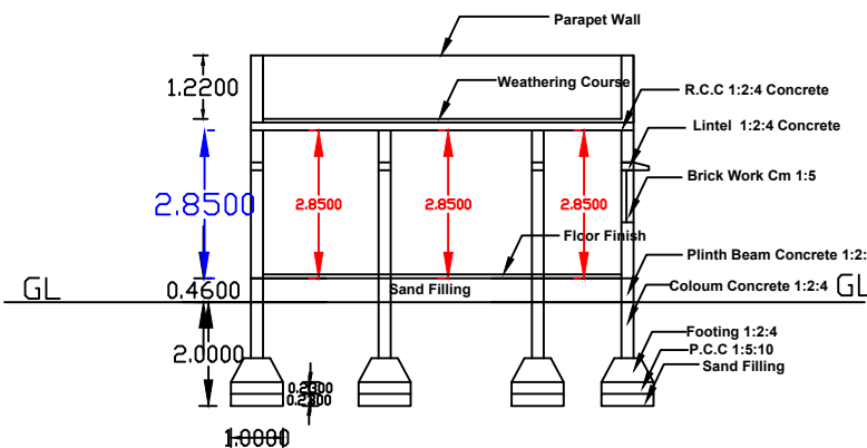
Section
