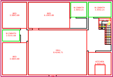
EXISTING GROUND FLOOR PLAN
