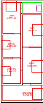
BUILT UP 862 SQ FT
