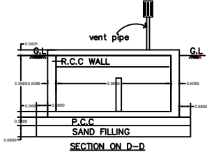
SECTION ON D-D
