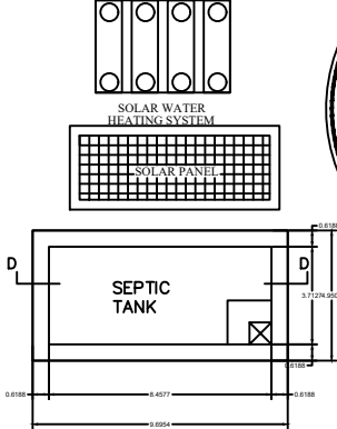
PLAN OF SEPTIC TANK SCALE 1"=2'-0"
