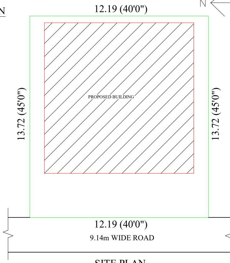
SITE PLAN
