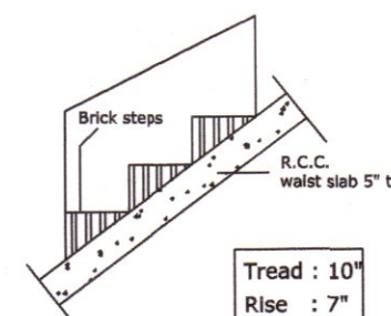
STAIRCASE DETAILS-nts
