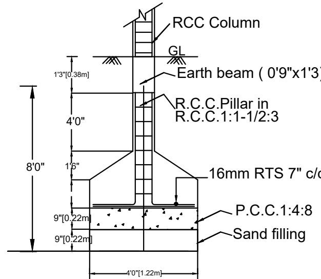
FOUNDATION DETAILS
