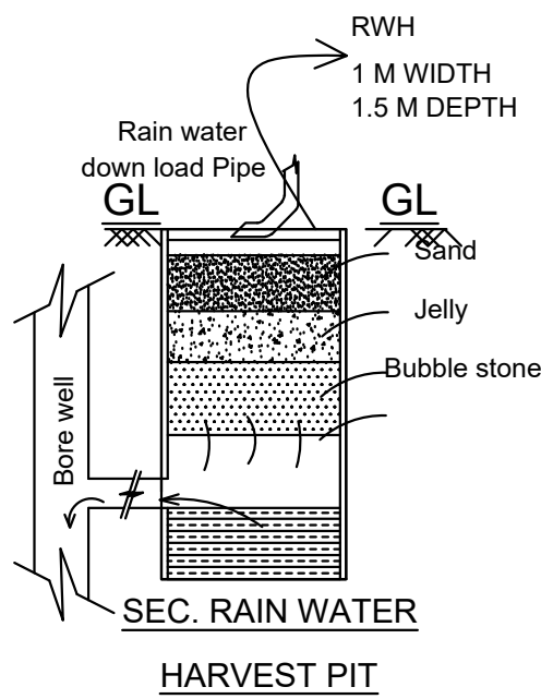
SEC. RAIN WATER HARVEST PIT
