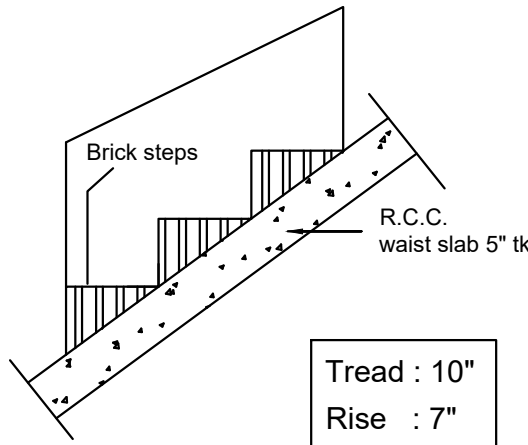
STAIRCASE DETAILS-nts
