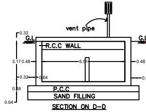
SECTION ON D-D
