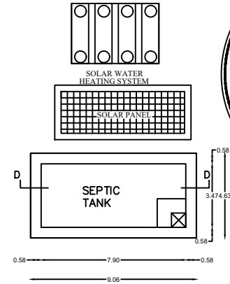
PLAN OF SEPTIC TANK SCALE 1"=2'-0"
