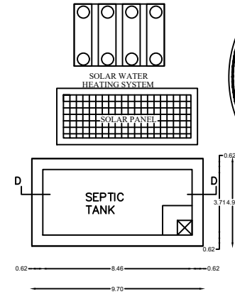
PLAN OF SEPTIC TANK SCALE 1"=2'-0"
