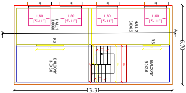
NON-RES FRIST FLOOR PLAN
