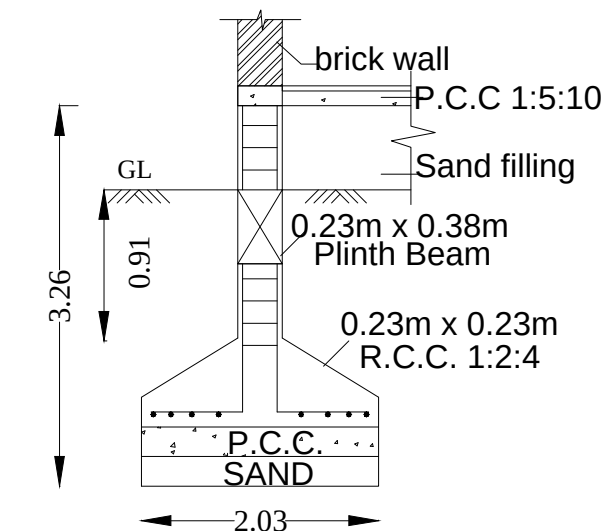
FOUNDATION DETAILS
