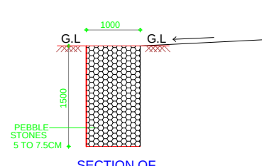
SECTION OF PEBBLE TRENCH
