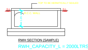
RWH_CAPACITY_L = 2000LTRS
