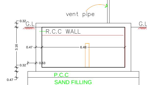
SECTION ON D-D
