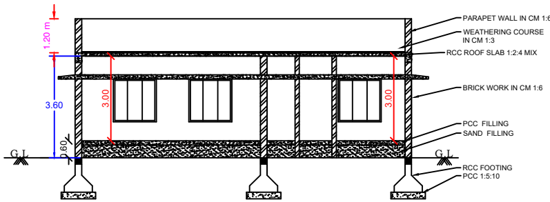
SECTION AB
