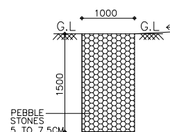
SECTION OF PEBBLE TRENCH SCALE : 1: = 100
