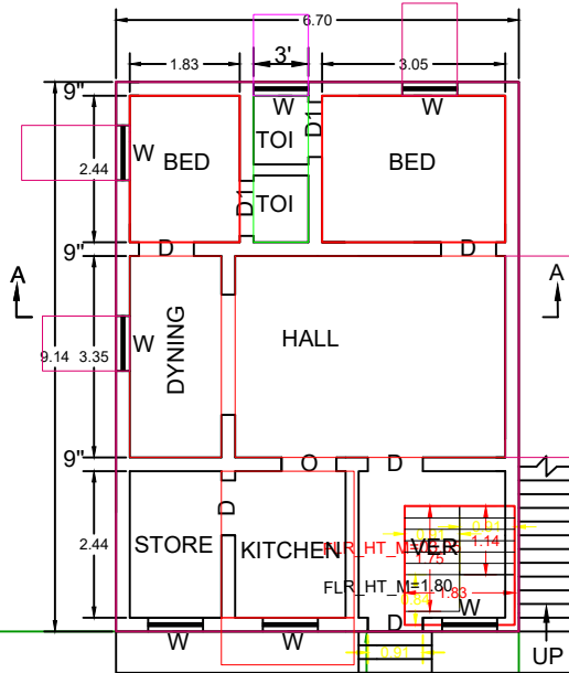
PROPOSED G.F. PLAN
