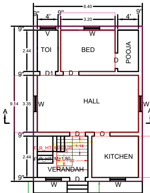
PROPOSED G.F. PLAN
