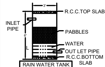
RAIN WATER TANK
