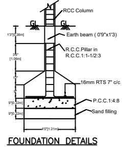
FOUNDATION DETAILS
