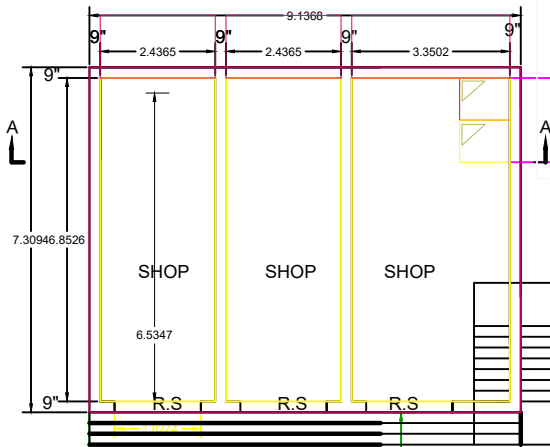
G.F. PLAN
