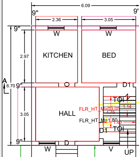
G.F. PLAN
