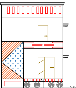
FRONT ELEVATION
