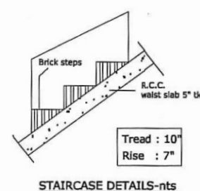
STAIRCASE DETAILS-nts
