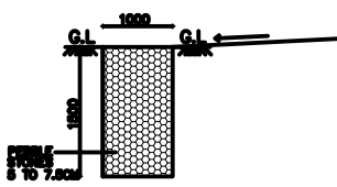
SECTION OF PEBBLE TRENCH SCALE : 1: = 100
