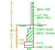
COMPOUND WALL DETAIL
