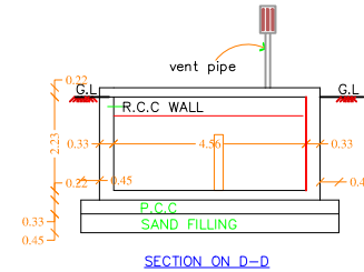
SECTION ON D-D
