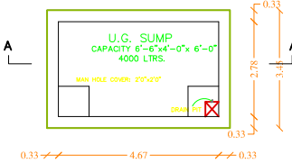
SUMP DETAIL SCALE 1"=4'-0"
