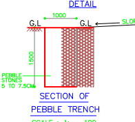
SECTION OF PEBBLE TRENCH SCALE 1:1 = 100
