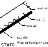
STAIR
