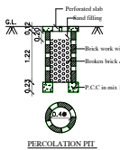
PERCOLATION PIT
