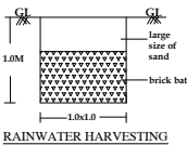
RAINWATER HARVESTING
