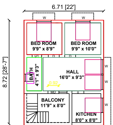
PRO.GROUND FLOOR
