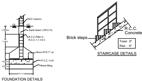
FOUNDATION DETAILS
