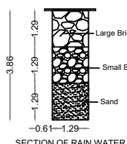
SECTION OF RAIN WATER COLLECTION PITS (NTS)
