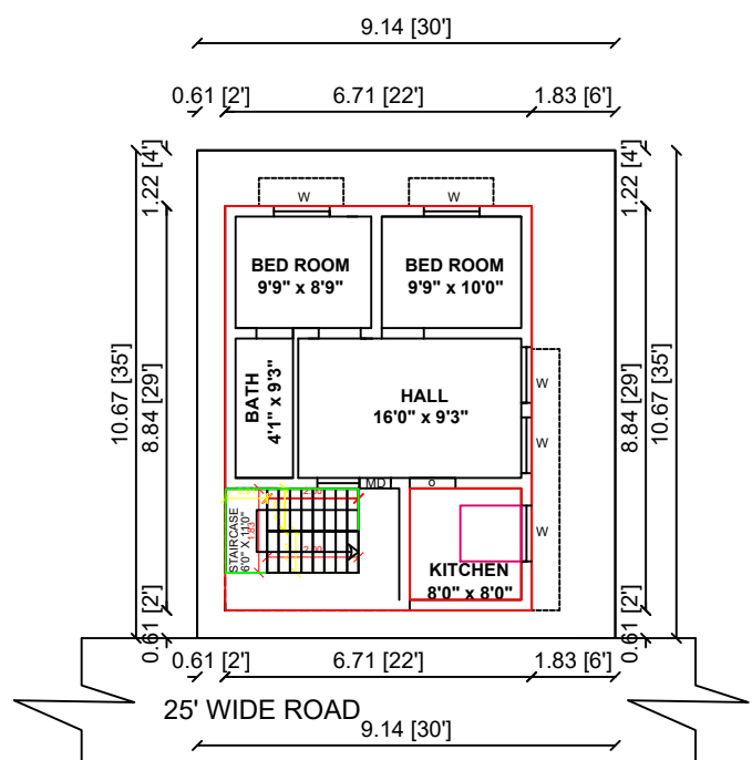
EXG.GROUND FLOOR
