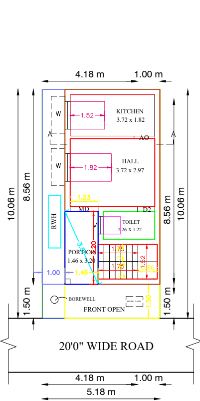
PRO.GROUND FLOOR PLAN
