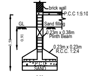
FOUNDATION DETAILS
