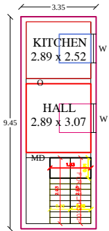
GROUND FLOOR PLAN
