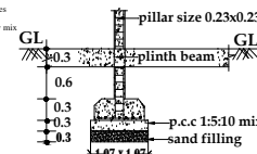
FOUNDATION DETAILS
