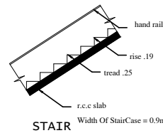
STAIR
