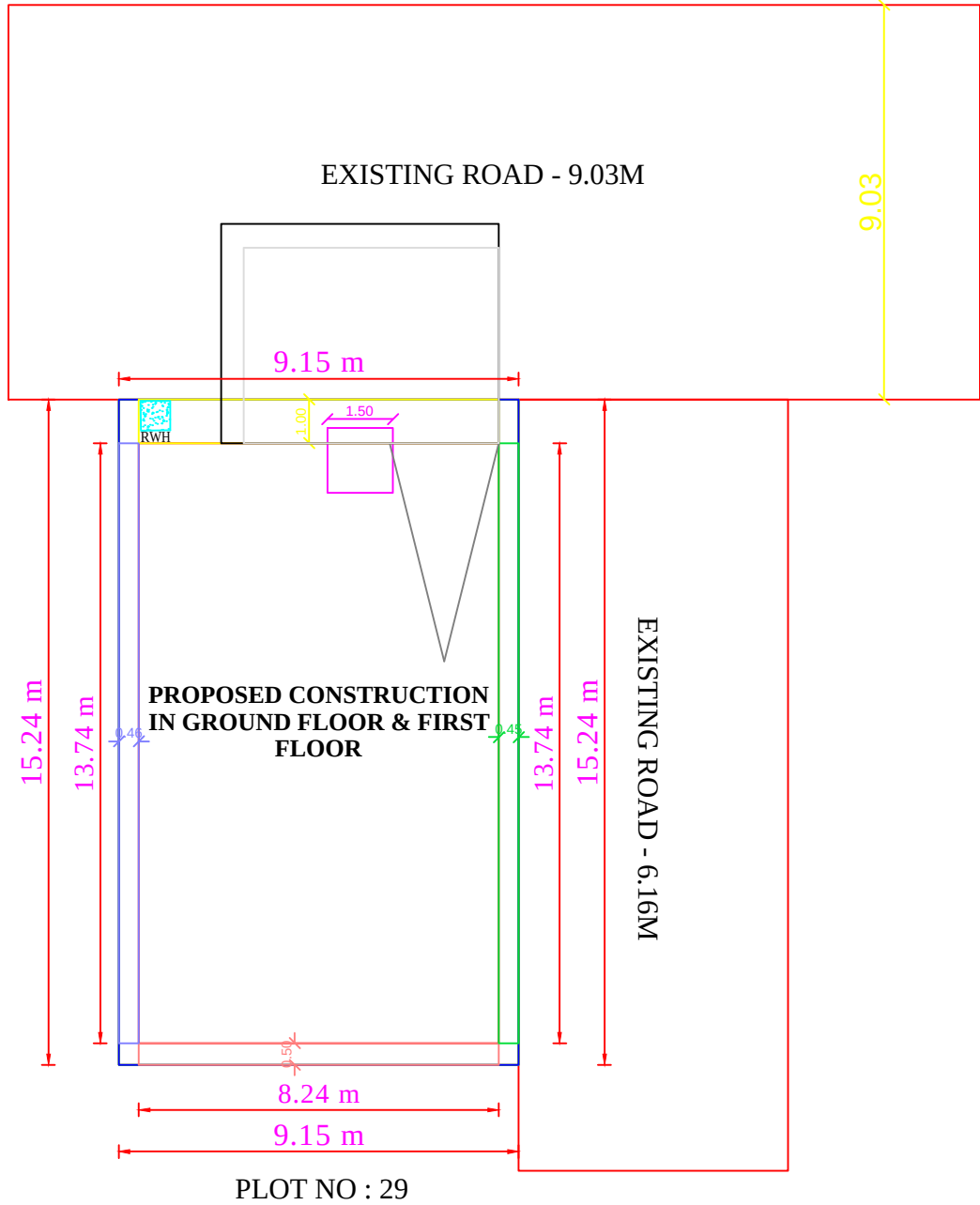
SITE PLAN
