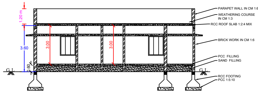
SECTION AB
