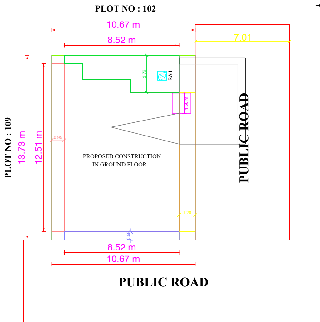
SITE PLAN
