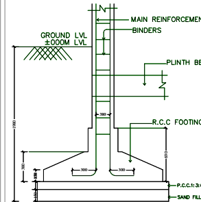
TYPICAL SECTION OF R.C.C. COLUMN FOUNDATION SCALE : 1" = 2'-0"
