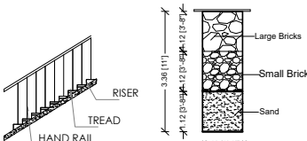
SECTION OF STAIR CASE DETAILS
