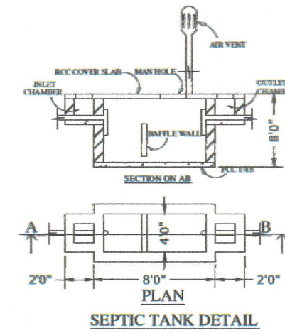
SEPTIC TANK DETAIL
