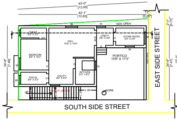
EXG., GROUND FLOOR PLAN
