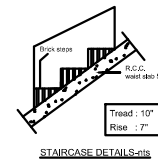
STAIRCASE DETAILS-etc
