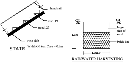
RAINWATER HARVESTING
