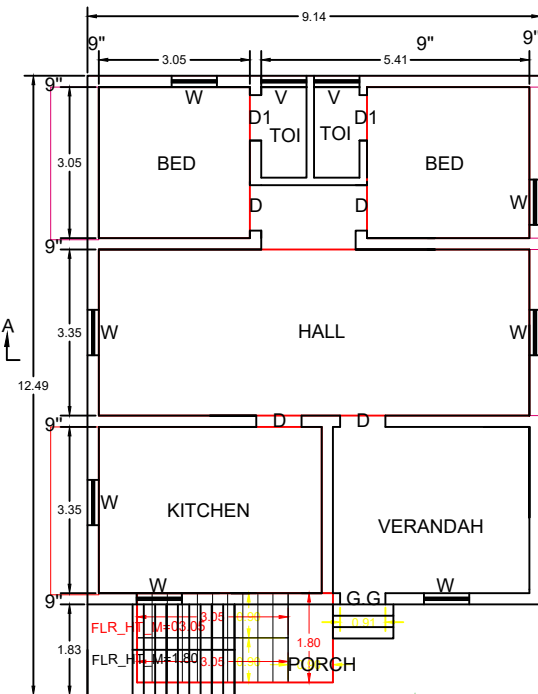
PROPOSED G.F. PLAN
