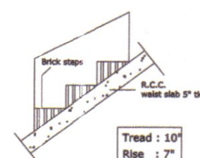
STAIRCASE DETAILS-nts
