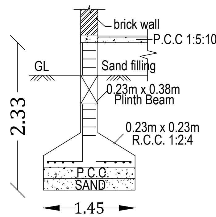
FOUNDATION DETAILS
