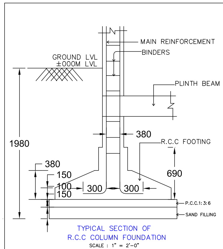
SECTION
