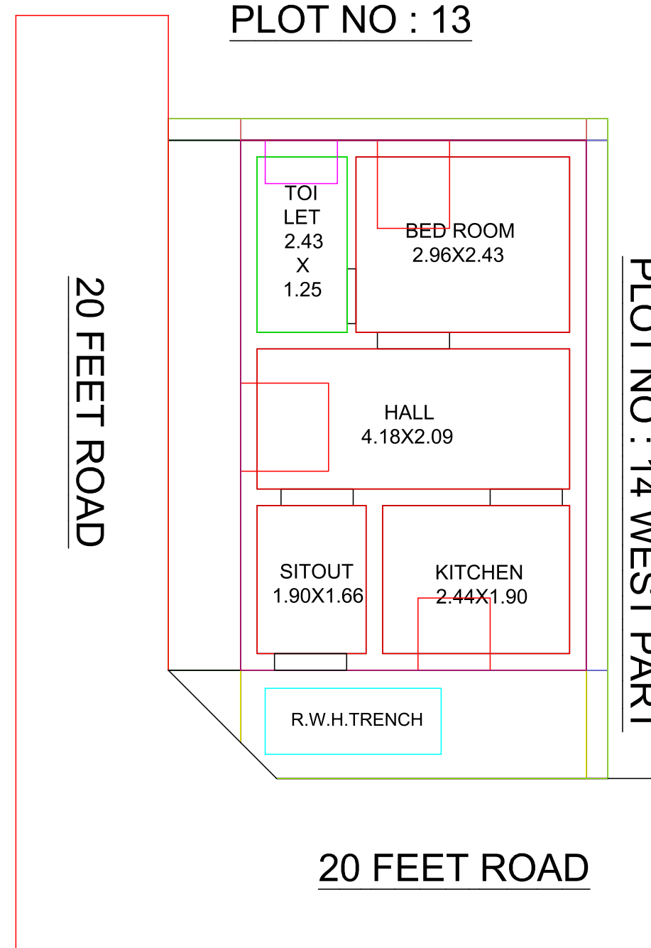
SITE PLAN
