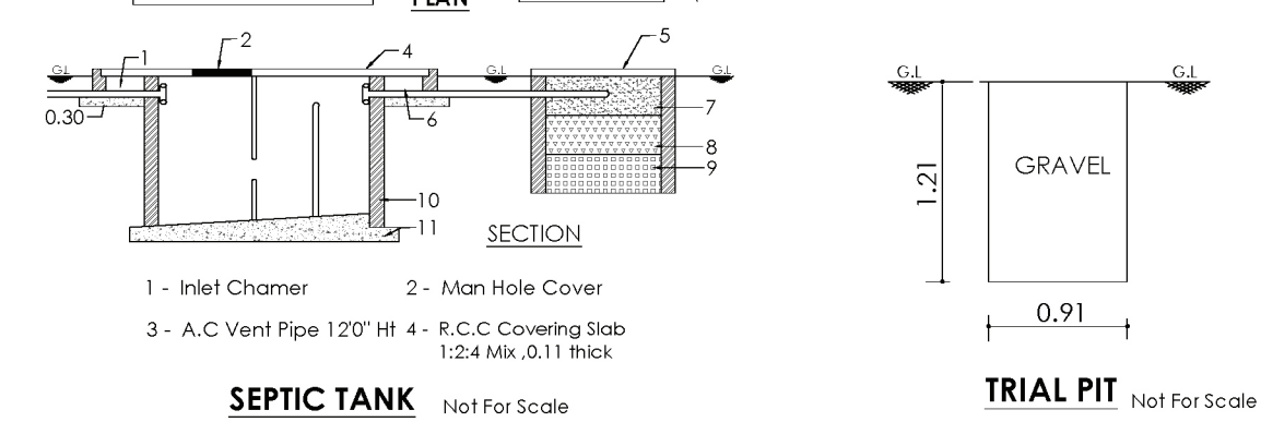
SEPTIC TANK
